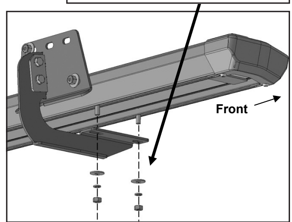
(Figure 10) Attach the driver/left Running Board to the front Mounting Bracket.
