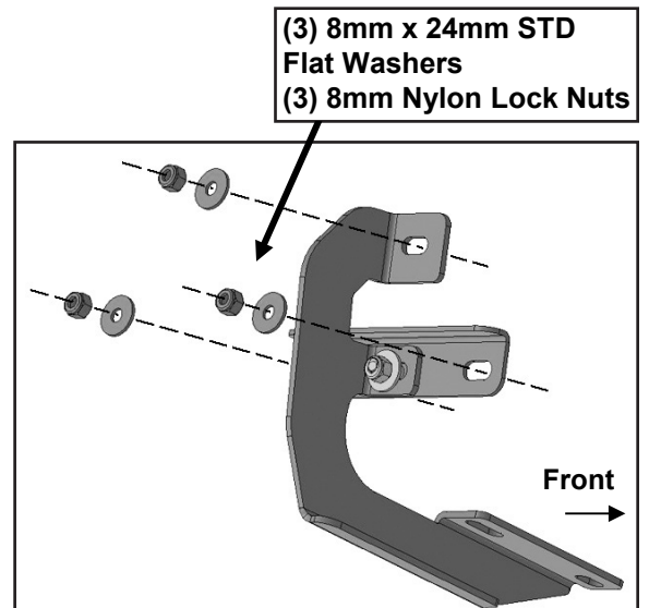
(Figure 7) Attach the center Bracket assembly to the (3) threaded studs in the center location.
