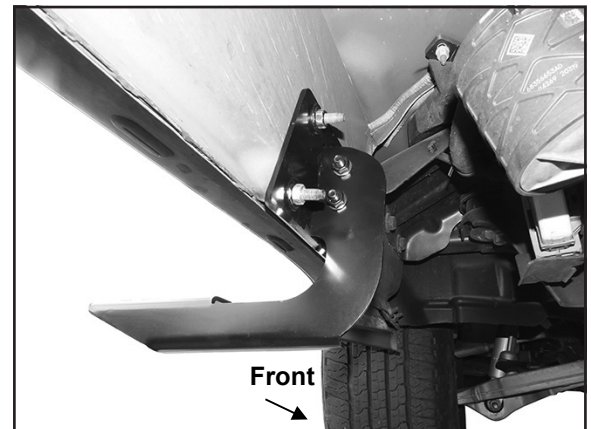
(Figure 4) Driver/left front Bracket assembly installed.
