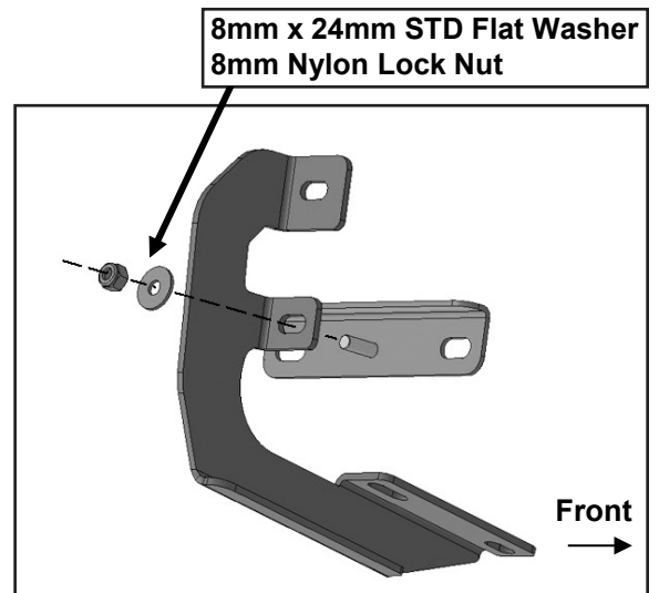
(Figure 6) Attach (1) Center Mounting Bracket to the threaded stud in (1) Support Bracket.
