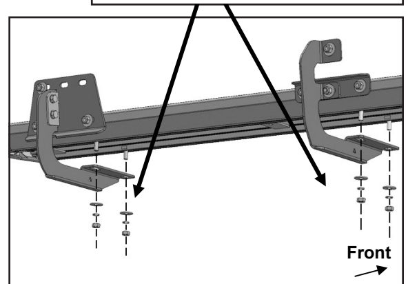
(Figure 12) Attach the driver/left Running Board to the center and rear Mounting Brackets.
