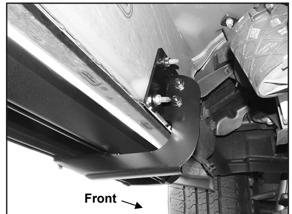
(Figure 11) Driver/left Running Board attached to the front Mounting Bracket.
