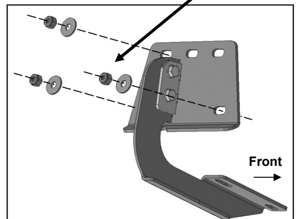
(Figure 3) Attach the front/rear Mounting Bracket assembly to the (3) threaded studs in the front mounting location.
