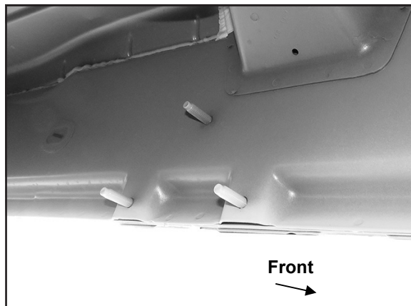
(Figure 5) Driver/left center mounting location.
