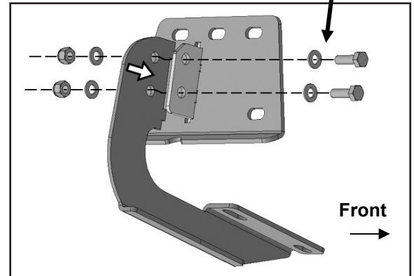
(Figure 2) Attach (1) front/rear Mounting Bracket to the back of (1) front/rear Mounting Plate.
